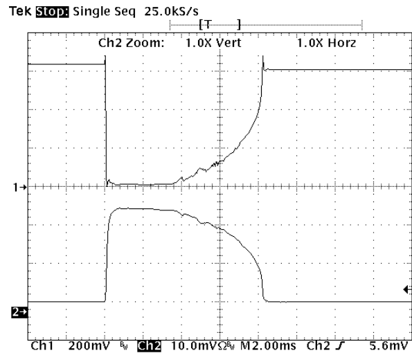
Fig. 11: Follow DC current interruption with experimental spark gap with DC extinguishing system in the circuit with condenser current source. U_{DC} = 600\text{ V} , I = 50\text{ A} , t_a = 8\text{ ms}
