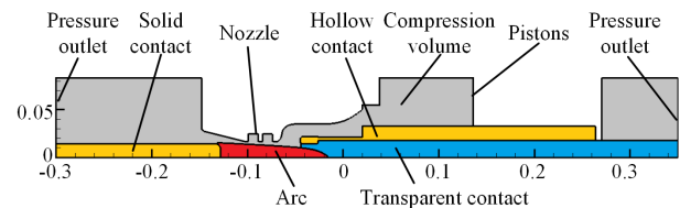
Figure 1. The simplified geometry and computational domain of the 252 kV puffer-type SF 6 circuit breakers
