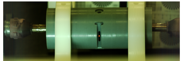
Figure 1. Experimental setup with PTFE nozzle. The observation window made of 2 mm thick quartz glass is positioned in the center of the PTFE nozzle. W-Cu electrodes at both sides are protected from exhaust plasma by ceramic caps.
